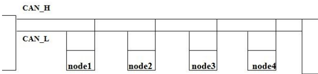
Fig. 8. The CAN Data Bus Lines.
